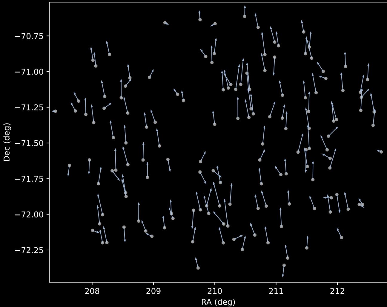
APOGEE DR17 Cluster 1 Proper Motion Vectors (n=143)
