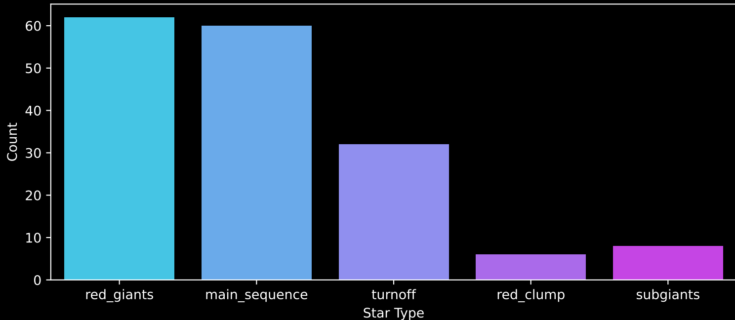
APOGEE DR17 Field: [283-23-O_TESS] Count plot of Star Type
