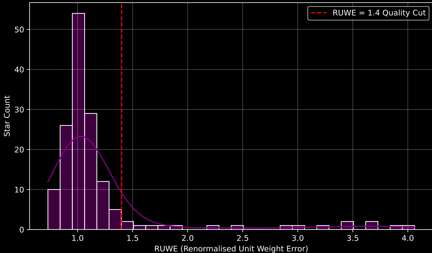
GAPOGEE DR17 Field [283-23-O_TESS] RUWE Distribution (n= 153)
